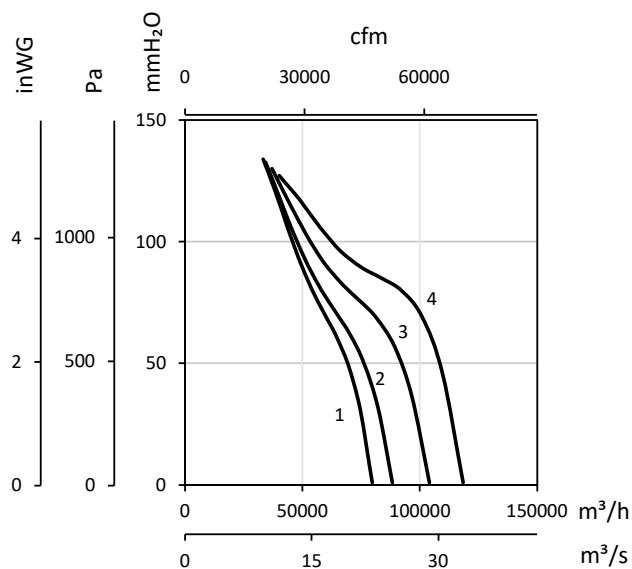
4T/9=1500 rpm
