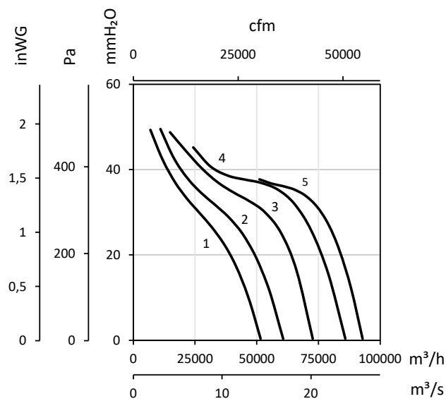
6T/6=1000 rpm
