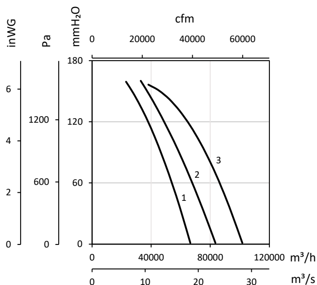
4T/12=1500 rpm
