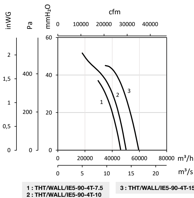
4T=1500 tr/min
