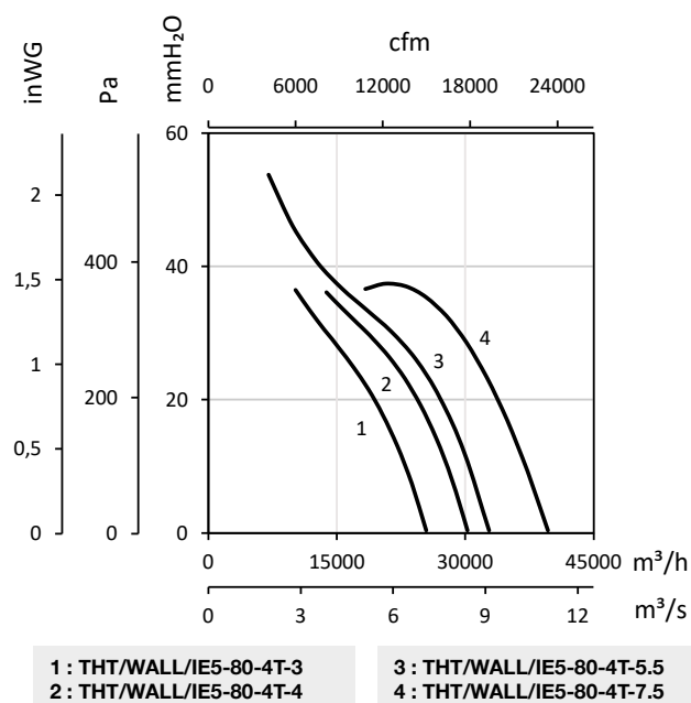
4T=1500 tr/min
